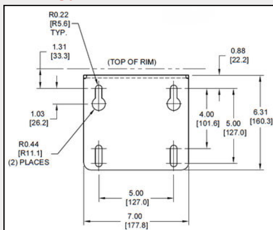
Mounting plate view: (Scale 2:1)
